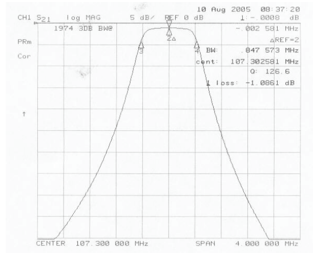
Rejection Plot 4-section filter
