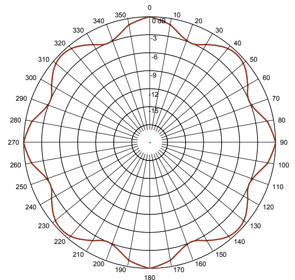
Standard 4 Round Omni Azimuth Pattern
